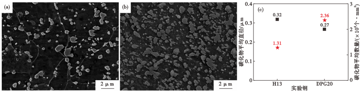
图6 实验钢球化退火后的微观组织及碳化物的统计结果:(a) H13 钢, (b) DPG20 钢, (c) 碳化物的统计结果 Fig. 6 Microstructure of experimental steels after spheroidizing annealing and statistical results of carbides : (a) H13 steel, (b) DPG20 steel, (c) statistical results of carbides
